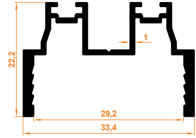
Düz Kapak Mentеше Profil Flat Cover with Hinge Profile
