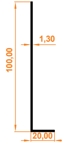
20x100 Köşebent 20x100 Angle Bracket
