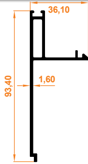
Kasa Kapatma Profili Frame Closure Profile
