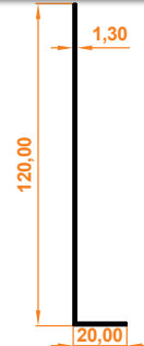
20x120 Köşebent 20x120 Angle Bracket
