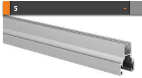
Küçük D Fitol Small D Wick Paket İçi Adet Amount within package 10 Gramajı Weight 0,167 kg/m
