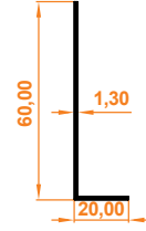
20x60 Köşebent 20x60 Angle Bracket
