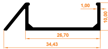
Junior Eşiksiz Kasa Profil Junior Case Profile without Threshold
