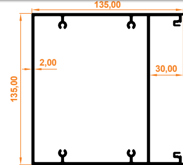
Gizli Ayak Profili Hidden Leg Profile
