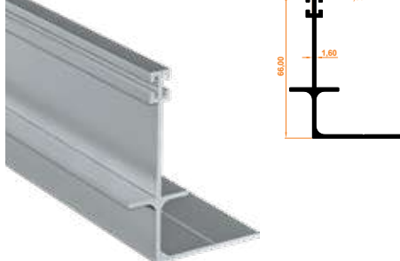
159 Açılımsız Çift Fitil Yan Ray L Kasa Profil Double Weatherstrips Without Opening Side L Case Profile
