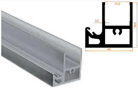
167 Kenet Baza Profil Clamp Base Profile
