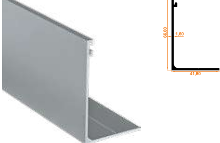
158 Açılımsız Tek Fitil Yan Ray L Kasa Profil Single Weatherstrips Without Opening Side L Case Profile
