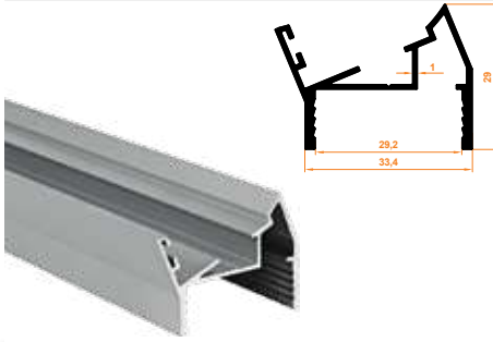
804 22,5° Dönüş Profil 22,5 degree Turn Profile
