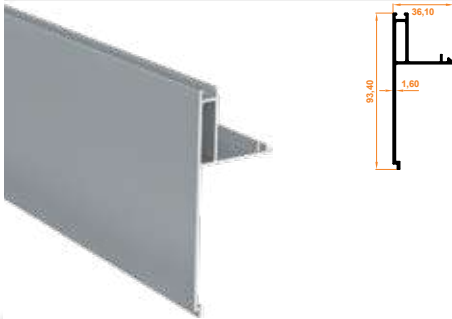
420 Kasa Kapatma Profili Frame Closure Profile
