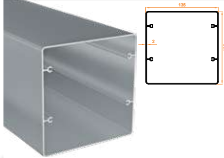
421 Ayak Profili Leg Profile
