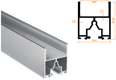
830 Fitilli Baza Profil Wick Base Profile
