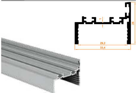
809 Sabit Cam Menteşe Profil Stable Glass Hinge Profile
