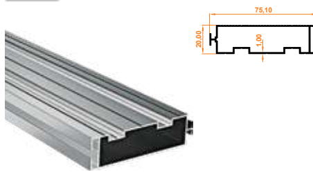
214 İkili Yan Kasa Profil Double Side Case Profile
