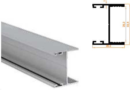
801 Düz Kapak Profil Flat Cover Profile
