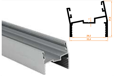
805 11° Dönüş Profil 11 degree Turn Profile
