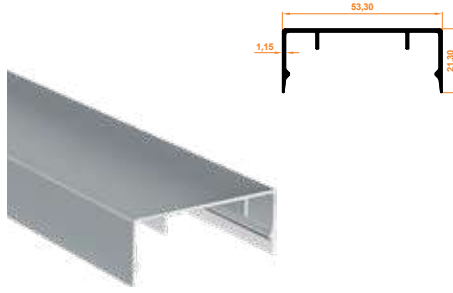
418 Cam Çita Kapak Profili Glass Strip Cover Profile
