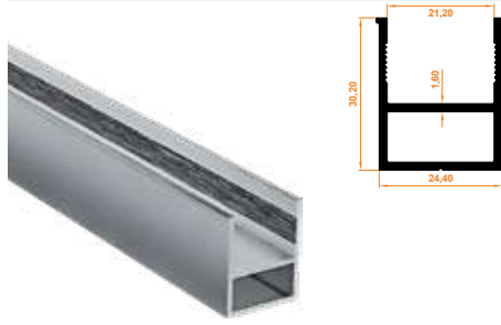
144 Hareketli Panel Yan Dikme Profil Movable Panel Side Column Profile
