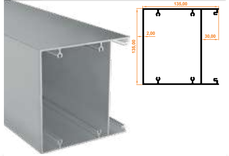
426 Gizli Ayak Profili Hidden Leg Profile
