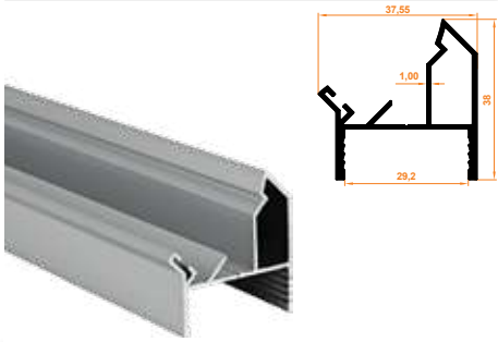
803 45° Dönüş Profil 45 degree Turn Profile
