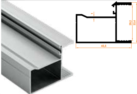
806 90° Dönüş Profil 90 degree Turn Profile
