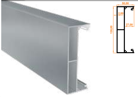
427 Destek Kutu Profili Reinforcing Box Profile
