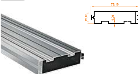
214 İkilü Yan Kasa Profil Double Side Case Profile
