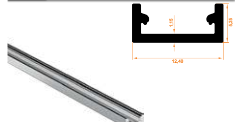
226 Kapatma Profil Closing Profile
