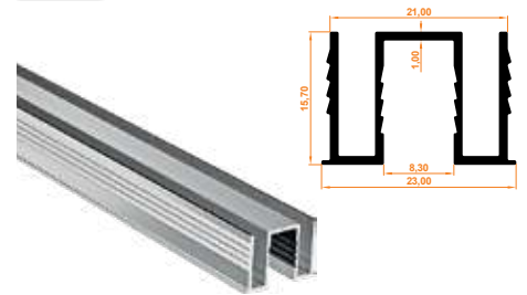
219 8 mm Cam Adaptörü 8 mm Glass Adapter
