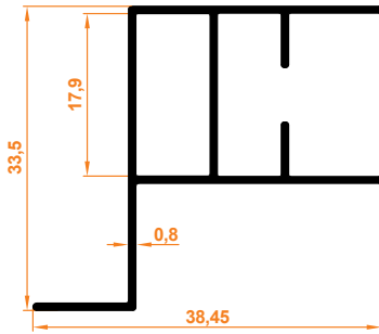
Kasa Profili Case Profile
