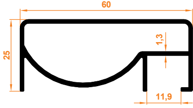
60x25 mm Üst Kúpeşte Yandan Kanallı 60x25 mm Upper Handrail with Side Channel
