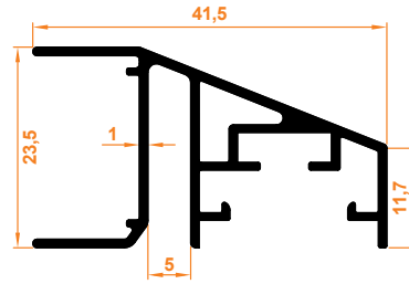
Plise Perde Kasa Profil Pleated Curtain Case Profile
