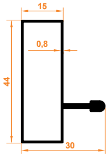
Platin Tekli Kasa Profil Platin Single Case Profile
