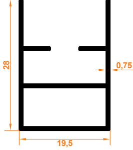
Slim Kasa Profili Slim Case Profile
