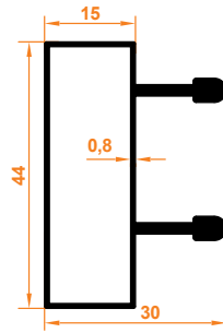
Platin Çiftli Kasa Profil Platin Double Case Profile
