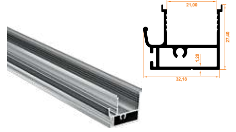
212 Kenet Profil Clamp Profile
