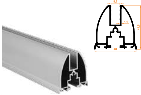
104 Gold Baza Profil Gold Base Profile
