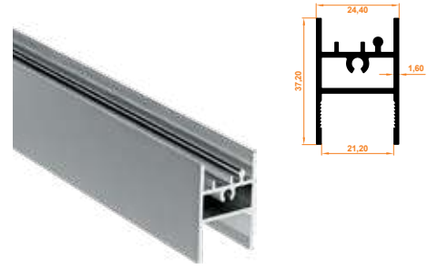
145 Kûpeşte Baza Profil Handrail Base Profile
