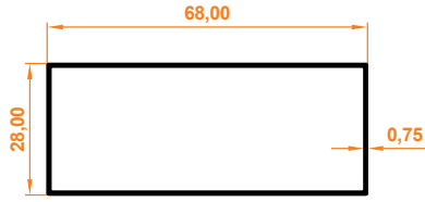
28x68 Kutu Profil 28x68 Box Profile
