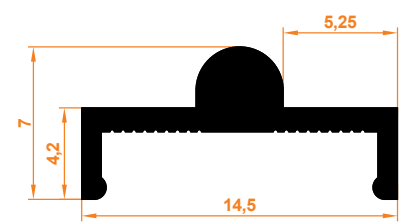
1532 Ray Profil 1532 Rail Profile
