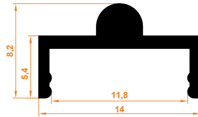
1531 Ray Profil 1531 Rail Profile
