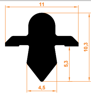
1064 Ray Profil 1064 Rail Profile
