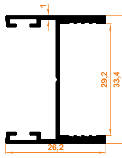
Düz Kapak Profil Flat Cover Profile
