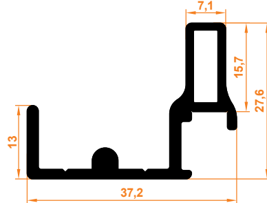
1575 Ray Profil 1575 Rail Profile
