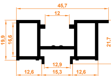
1553 Ray Profil 1553 Rail Profile
