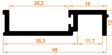
1572 Ray Profil 1572 Rail Profile
