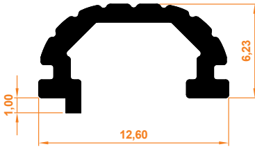
Yaylı Portray Profil Spring Portray Profile
