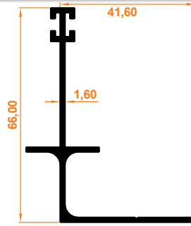
Açılımsız Çift Fitol Yan Ray L Kasa Profil Double Weatherstrips Without Opening Side L Case Profile
