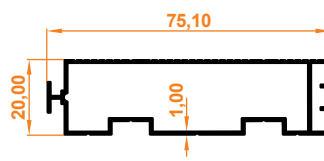
İkili Yan Kasa Profil Double Side Case Profile
