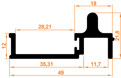
1571 Ray Profil 1571 Rail Profile
