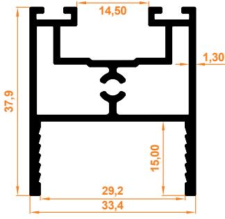
Fıllı Baza Profil Wicked Base Profile
