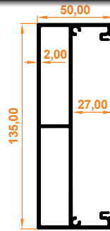
Destek Kutu Profili Reinforcing Box Profile
