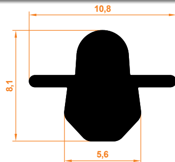
1560 Ray Profil 1560 Rail Profile
