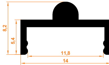
1531 Ray Profil 1531 Rail Profile
