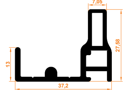
1576 Ray Profil 1576 Rail Profile
