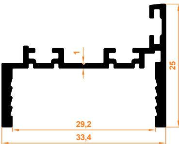
Sabit Cam Mentşe Profil Stable Glass Hinge Profile
