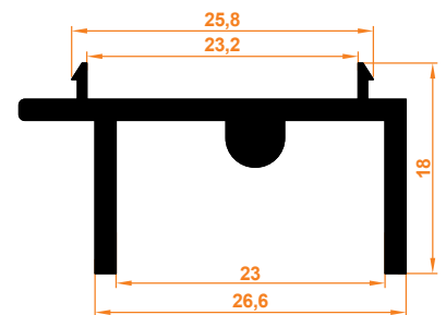
1552 Ray Profil 1552 Rail Profile
