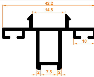
1063 Ray Profil 1063 Rail Profile
