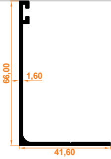
Açılımsız Tek Fitol Yan Ray L Kasa Profil Single Weatherstrips Without Opening Side L Case Profile
