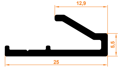
1573 Ray Profil 1573 Rail Profile
