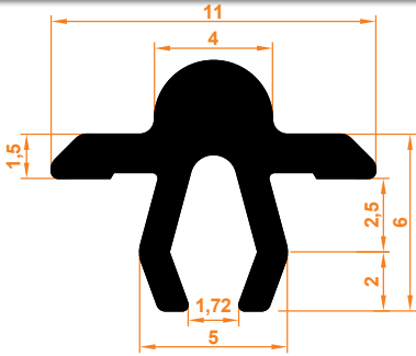
1002 Ray Profil 1002 Rail Profile
