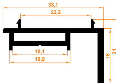
1551 Ray Profil 1551 Rail Profile
