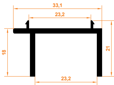
1550 Ray Profil 1550 Rail Profile
