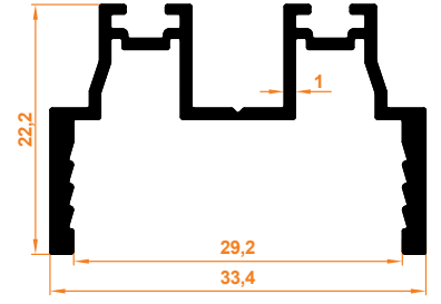
Düz Kapak Mentşe Profil Flat Cover with Hinge Profile
