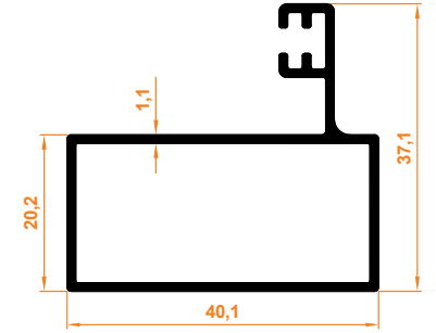
Geniş Yan Dikme Thick Side Column Profile
