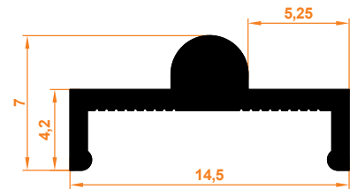
1532 Ray Profil 1532 Rail Profile
