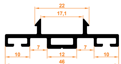
1570 Ray Profil 1570 Rail Profile
