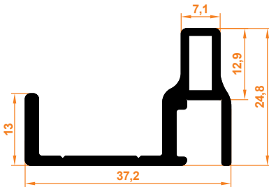
1577 Ray Profil 1577 Rail Profile
