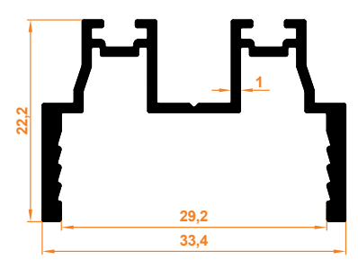
Düz Kapak Mentеше Profil Flat Cover with Hinge Profile
