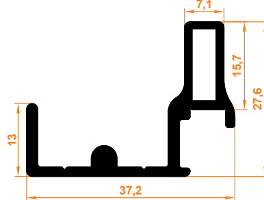
1575 Ray Profil 1575 Rail Profile
