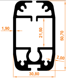
Kanat Profili Wing Profile
