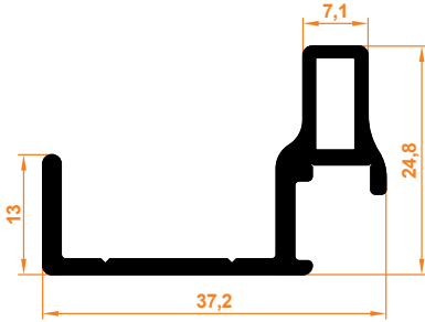
1574 Ray Profil 1574 Rail Profile
