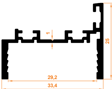
Sabit Cam Mentеше Profil Stable Glass Hinge Profile
