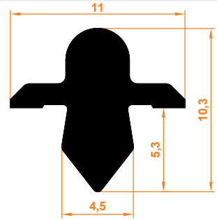
1064 Ray Profil 1064 Rail Profile
