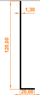
20x120 Köşebent 20x120 Angle Bracket
