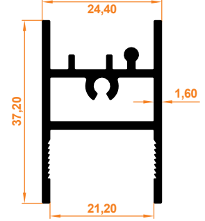
Kúpeşte Baza Profil Handrail Base Profile
