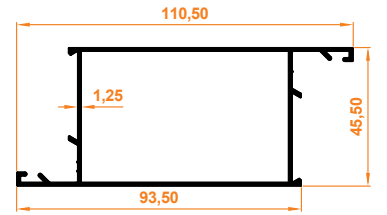
Aldoks (Geniş) Kanat Profili Aldoks (Wide) Wing Profile
