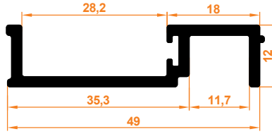
1572 Ray Profil 1572 Rail Profile
