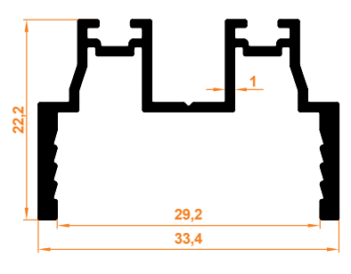
Düz Kapak Mantese Profili Flat Cover with Hinge Profile
