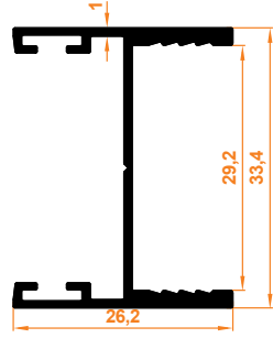
Düz Kapak Profili Flat Cover Profile
