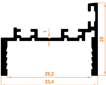
Sabit Cam Mantese Profili Stable Glass Hinge Profile
