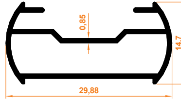
Aura Alt Kasa Profili Aura Buttom Case Profile
