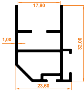
Plise Perde Kasa Profil Pleated Blind Casing Profile
