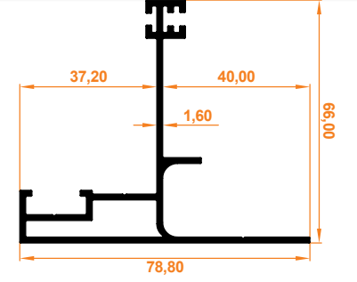
Yan Ray "T" Profil Side Rail "T" Profile
