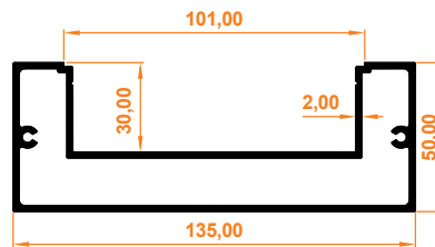
Destek Kutu Profili Reinforcing Box Profile
