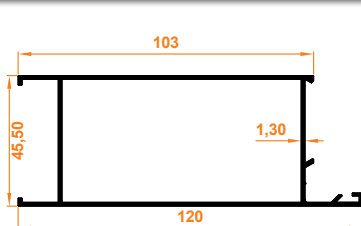
Aldoks Etek Profili Aldoks Skirt Profile
