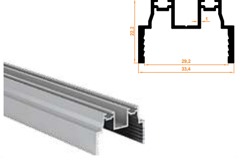
802 Düz Kapak Menteşe Profil Double Glass Flat Cover with Hinge Profile
