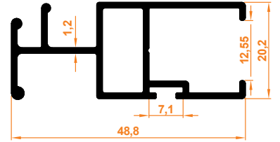
Platin Kanat Profil Platin Series Sash Profile
