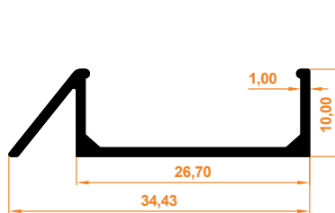
Junior Eşiksiz Kasa Profil Junior Case Profile without Threshold
