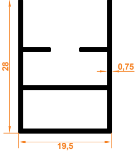
Slim Kasa Profil Slim Case Profile
