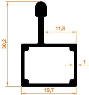
Platin Tekli Dar Kasa Profil Platin Series Single Slim Frame Profile
