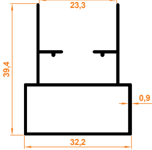
Gold Kasa Profil Gold Case Profile
