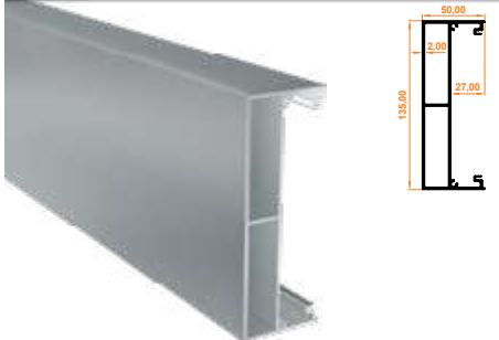
427 Destek Kutu Profili Reinforcing Box Profile
