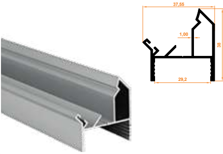
803 45° Dönüş Profil 45 degree Turn Profile
