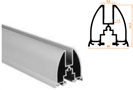
104 Gold Baza Profil Gold Base Profile gold
