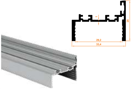
809 Sabit Cam Mentеше Profil Stable Glass Hinge Profile
