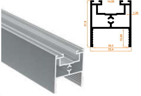
829 Fitilli Baza Profil Wicked Base Profile
