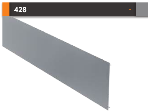
Gizli Ayak ve Destek Kutu Kapatma Profili Hidden Leg Case Cover Support Profile Paket İçi Adet Quantity Per Package 10 Gramajı Weight 0,501 kg/m
