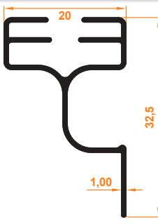
Etekli 20'lik T Profil Skirted 20 T Profile
