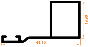
Kasa Profil Case Profile
