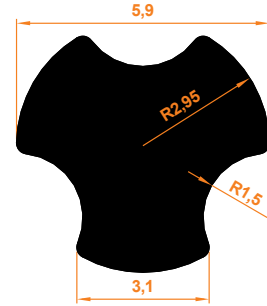
Zebra Dikey Mil Vertical Shaft for Zebra Blinds
