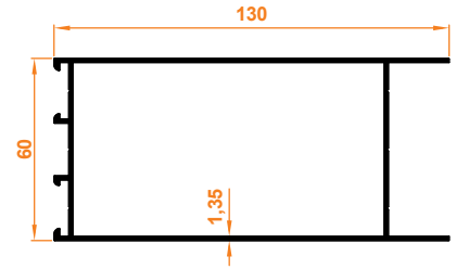
C60 Etek Profili C60 Skirt Profile
