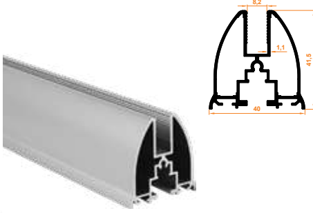
104 Gold Baza Profil Gold Base Profile
