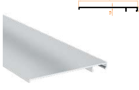
177 Küşte Profil Handrail Profile
