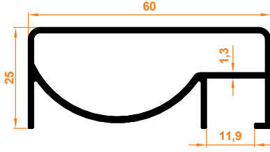
60x25 mm Üst Kúpeşte Yandan Kanallı 60x25 mm Upper Handrail with Side Channel
