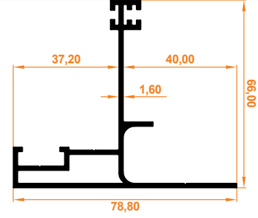
Yan Ray "T" Profil Side Rail "T" Profile
