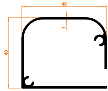
Stor Kasa Profil Stor Case Profile
