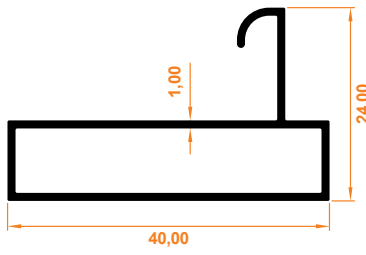
Stor Alt Kasa Profil Stor Bottom Case Profile
