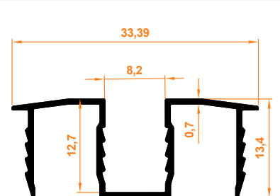
8 mm Cam Adaptörü 8 mm Glass Adapter
