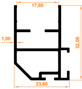
Plise Perde Kasa Profili Pleated Blind Casing Profile
