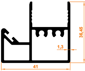
Kenet Baza Profil Interlocking Base Profile
