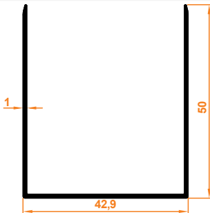
U Kapatma Profil U Closing Profile
