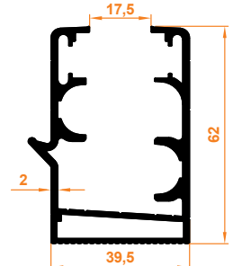
Oluklu Kasa Profili Corrugated Case Profile
