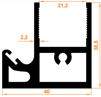
Kenet Baza Profil Clamp Base Profile
