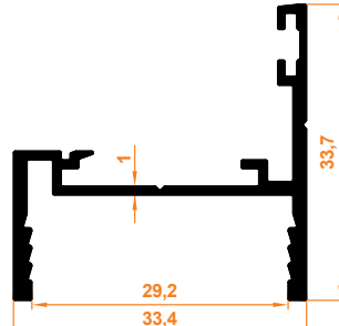
Sabit Cam (Tijli) Kilit Profili Stable Glass Lock Profile
