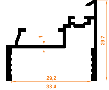
Sabit Cam (Tijli) Kilit Karşılık Profili Stable Glass Lock Prevention Profile
