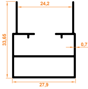
Star Kasa Profil Star Case Profile
