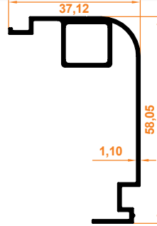
Ray Kapatma "T" Profil Rail Closure "T" Profile
