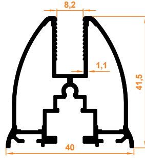
Gold Baza Profil Gold Base Profile
