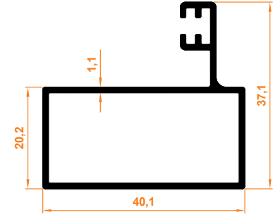
Geniş Yan Dikme Thick Side Column Profile
