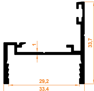
Sabit Cam Kilit Profili Stable Glass Lock Profile
