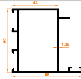
C60 Kanat Profili C60 Wing Profile
