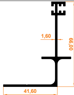
Yan Ray "L" Profil Side Rail "L" Profile
