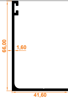
Açılımsız Tek Fitil Yan Ray L Kasa Profil Single Weatherstrips Without Opening Side L Case Profile
