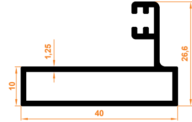
Dar Yan Dikme Thin Side Column
