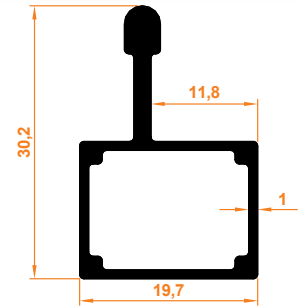
Platin Tekli Slim Kasa Profil Platin Single Case Slim Profile
