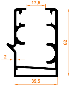
Oluklu Kasa Profili Corrugated Case Profile
