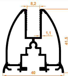
Gold Baza Profil Gold Base Profile
