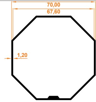
Sac Tambur Borusu Sheet Metal Drum Tube
