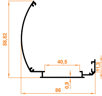
Kapalı Kasa Geniş Profil Wide Closed-Case Profile
