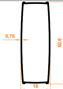
Ahşap Jaluzi Perde Etek Profil Venetian Blind Bottomrail Profile
