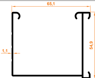
Ahşap Jaluzi Perde Kasa Profil Venetian Blind Headrail Profile
