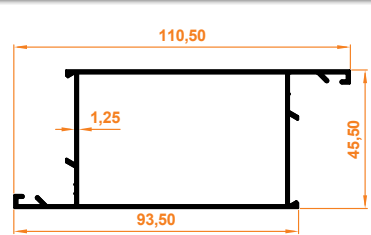
Aldoks (Geniş) Kanat Profili Aldoks (Wide) Wing Profile
