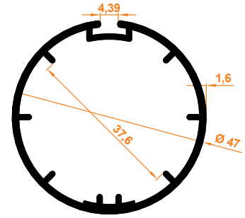
Zebra Perde 47'lik Motor Boru Zebra Blind Ø47 Motor Tube
