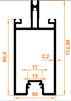
Ledli Orta Kayıt Profili Center Mullion Profile with Led
