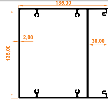
Gizli Ayak Profili Hidden Leg Profile
