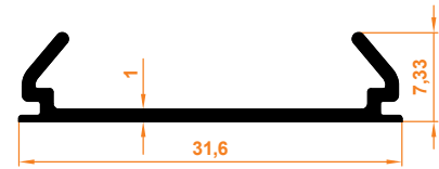
Kapatma Profil Closing Profile
