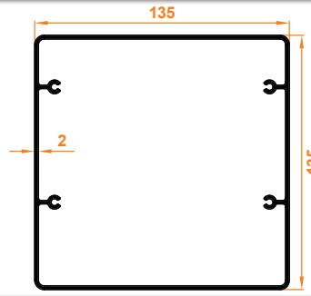
Ayak Profili Aluminium Pfosten
