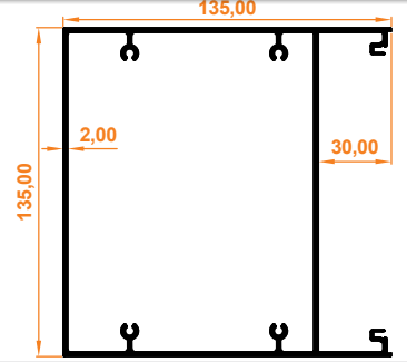
Gizli Ayak Profili Hidden Leg Profile
