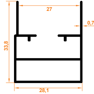
Star Kasa Profil Star Case Profile
