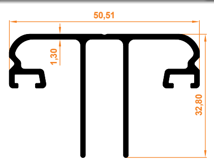
Cam Çita Profili Glass Strip Profile
