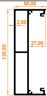
Destek Kutu Profili Reinforcing Box Profile
