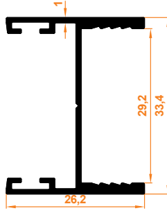
Düz Kapak Profili Flat Cover Profile
