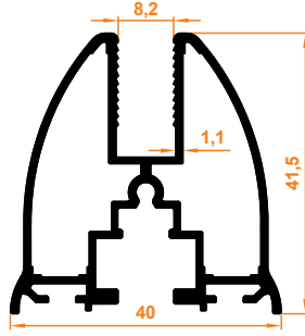
Gold Baza Profil Gold Base Profile
