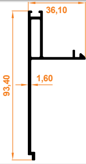
Kasa Kapatma Profili Frame Closure Profile
