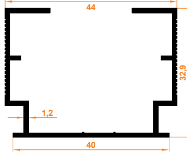
Dikey Geniş Kasa Vertical Wide Headbox
