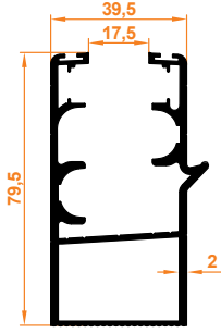
Üstten Fitilli Büyük Oluklu Kasa Large Corrugated Case with Top Wick
