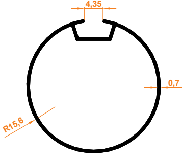
32'lik Boru Ø32 Roller Tube
