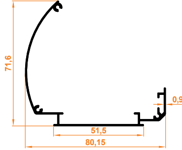
Zebra Perde Kapalı Kasa Closed Cassette for Zebra Blinds
