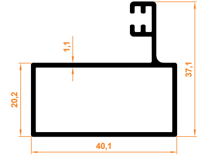
Geniş Yan Dikme Thick Side Column Profile
