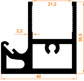
Kenet Baza Profil Clamp Base Profile
