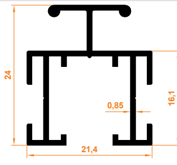
Çiftli Orta Profil Double Middle Profile
