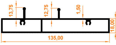
Alt Kasa Guillotine Lower Case Profile
