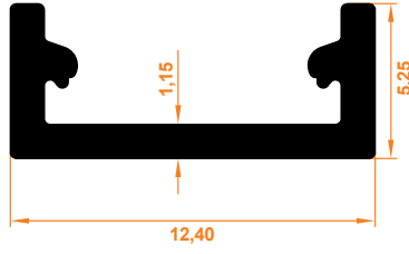
Kapatma Profil Closing Profile
