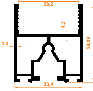
Fitilli Baza Profili Wicked Base Profile
