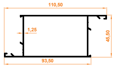
Aldoks (Geniş) Kanat Profili Aldoks (Wide) Wing Profile
