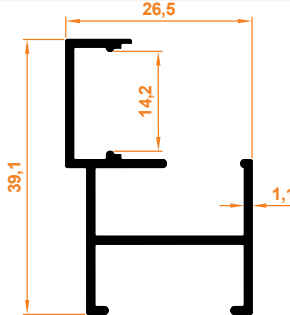
Cam Tutucu Profil Glass Holder Profile
