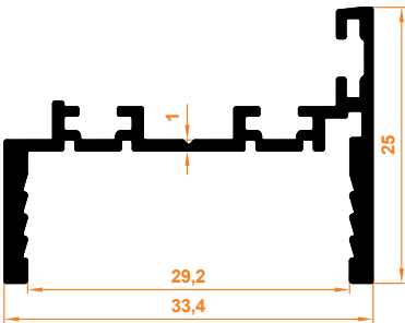
Sabit Cam Menteşe Profili Stable Glass Hinge Profile
