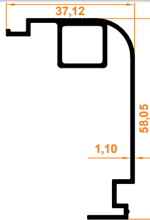
Ray Kapatma "T" Profil Rail Closure "T" Profile
