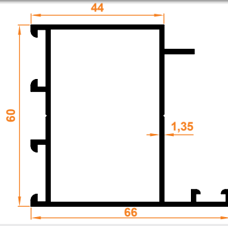
C60 Kanat Profili C60 Wing Profile
