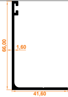
Açılımsız Tek Fıtil Yan Ray L Kasa Profil Single Weatherstrips Without Opening Side L Case Profile
