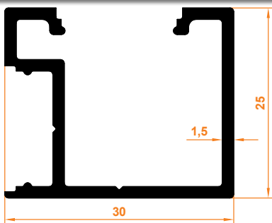
Takviyesiz Cam Tutucu Profil Non-Reinforced Glass Holder Profile
