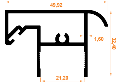
Sabit Panel Üst Baza Profil Fixed Panel Top Base Profile
