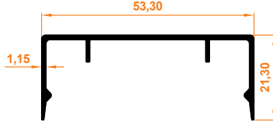
Cam Çita Kapak Profili Glass Strip Cover Profile
