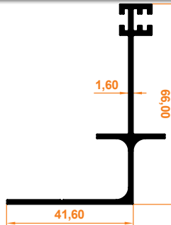
Yan Ray "L" Profil Side Rail "L" Profile
