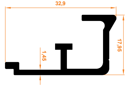
Yan Kasa Kapak Profili Side Case Cover Profile
