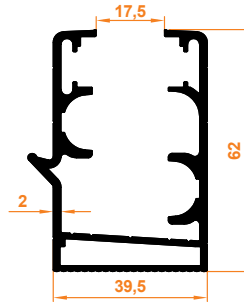
Oluklu Kasa Profil Corrugated Case Profile
