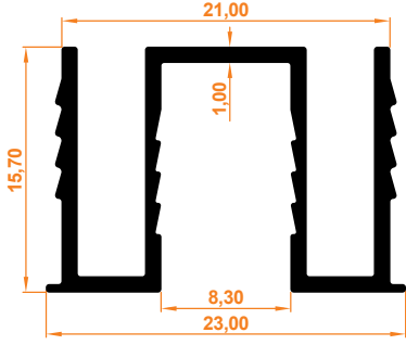
8 mm Cam Adaptörü 8mm Glass Adapter
