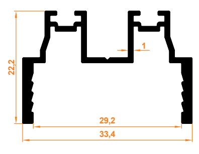
Düz Kapak Menteşe Profili Flat Cover with Hinge Profile
