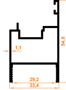
Sabit Cam İspanyolet Profil Fixed Glass Espagnolette Profile
