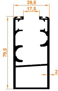
Üstten Fitilli Büyük Düz Kasa Large Flat Case with Wed from Top
