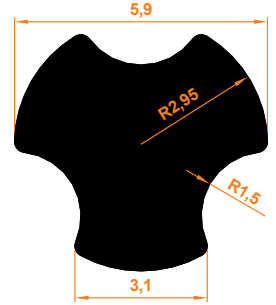
Zebra Dikey Mil Vertical Shaft for Zebra Blinds
