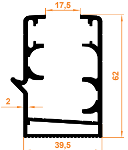
Oluklu Kasa Profili Corrugated Case Profile
