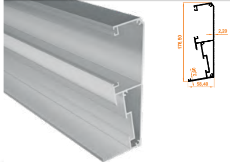
424 Duvar Kasa Profili Wall Frame Profile
