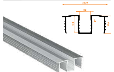
126 8 mm Cam Adaptörü 8 mm Glass Adapter
