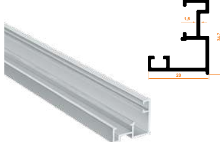
180 Yan Karşılık Profil Side Counterpart Profile
