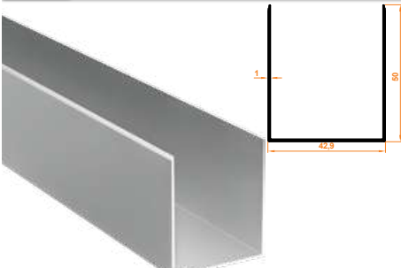
932 U Kapatma Profil U Closing Profile
