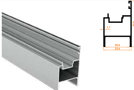
824 Sabit Cam İspanolet Profil Fixed Glass Espagnolette Profile
