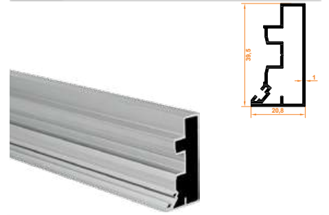
808 Isıcam Yan Dikme Profil Double Glass Side Column Profile
