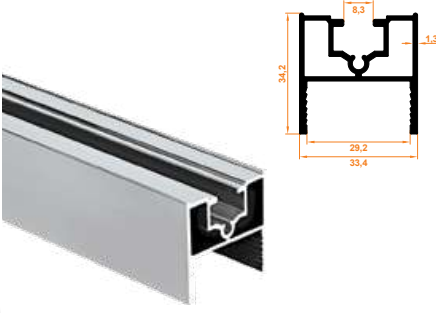
800 Baza Profil Double Glass Base
