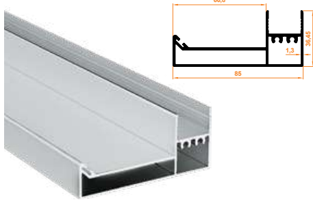
173 Geniş Kenet Baza Profil Wide Interlocking Base Profile
