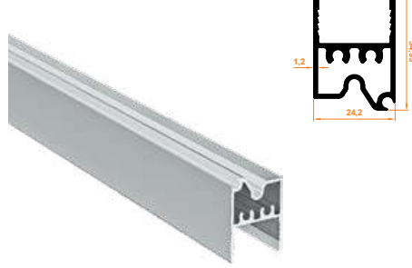
171 Bitim Baza Profil End Base Profile
