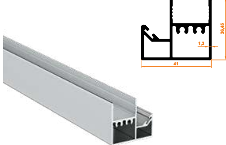
176 Kenet Baza Profil Interlocking Base Profile
