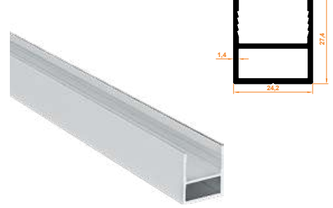
172 Dikme Profil Mullion Profile
