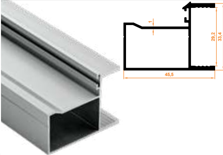
806 90° Dönüş Profil 90 degree Turn Profile
