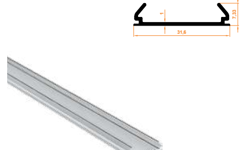
175 Kapatma Profil Closing Profile
