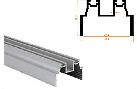
802 Düz Kapak Menteşe Profil Double Glass Flat Cover with Hinge Profile
