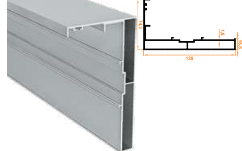
181 Yan Kasa Profil Side Frame Profile
