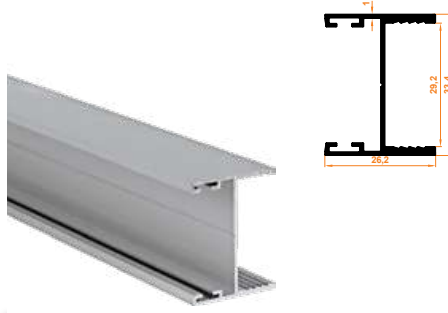
801 Düz Kapak Profil Double Glass Flat Cover Profile
