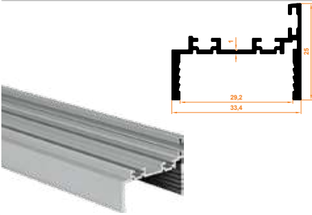
809 Sabit Cam Menteşe Profil Stable Glass Hinge Profile
