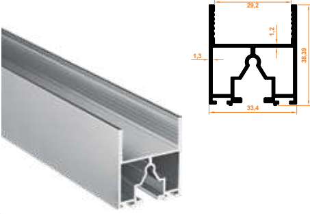
830 Fitilli Baza Profil Wick Base Profile
