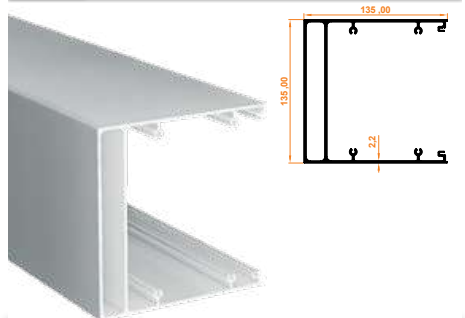
432 Gizli Ayak Profili Hidden Leg Profile
