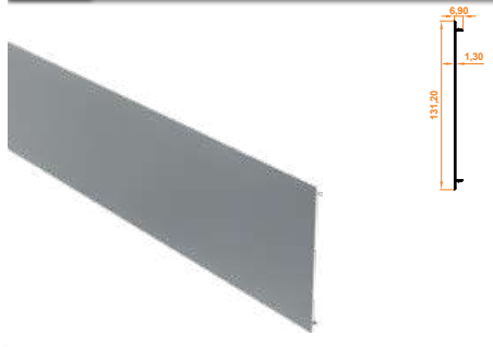
428 Gizli Ayak ve Destek Kutu Kapatma Profili Hidden Leg Case Cover Support Profile
