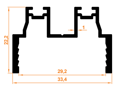
Düz Kapak Menteşe Profil Flat Cover with Hinge Profile
