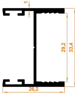
Düz Kapak Profil Flat Cover Profile
