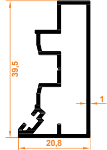
Yan Dikme Profil Side Column Profile
