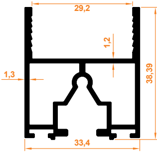
Fitilli Baza Profil Wicked Base Profile
