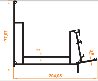
Mukavemetli Oluk Profil Reinforced Groove Profile
