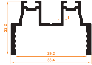
Düz Kapak Menteşe Profili Flat Cover with Hinge Profile
