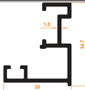
Yan Karşılık Profil Side Counterpart Profile
