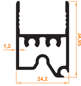
Bitim Baza Profil End Base Profile
