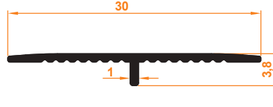
T Profili T Profile
