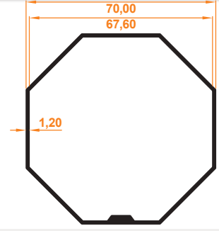
Sac Tambur Borusu Sheet Metal Drum Tube
