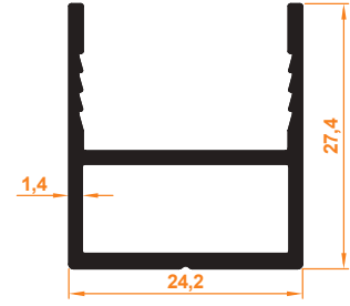
Dikme Profil Mullion Profile
