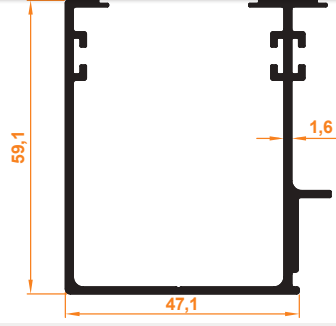
Yan U Profil Side U Profile
