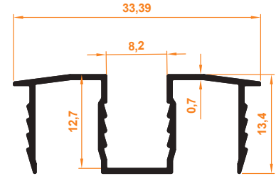
8 mm Cam Adaptörü 8 mm Glass Adapter
