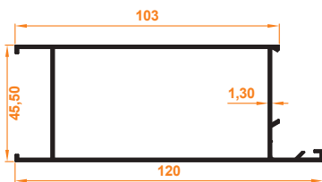
Aldoks Etek Profili Aldoks Skirt Profile
