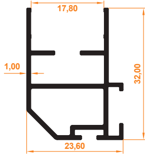
Plise Perde Kasa Profili Pleated Blind Casing Profile
