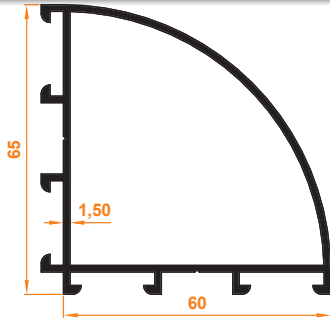
C60 Oval Köşe Dönüş Profili C60 Oval Corner Profile
