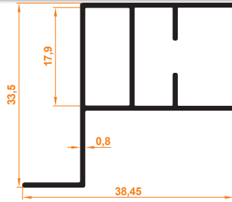
Slim Seri İçten Montajlı Kasa Profil Slim Series Internally Mounted Frame Profile
