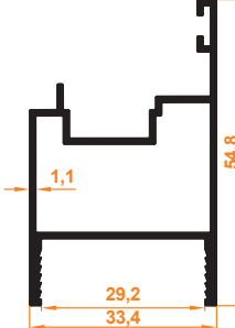
Sabit Cam İspanyolet Profil Fixed Glass Espagnolette Profile
