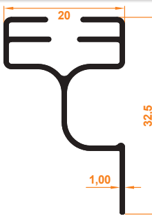
Etekli 20'lik T Profil Skirted 20 T Profile
