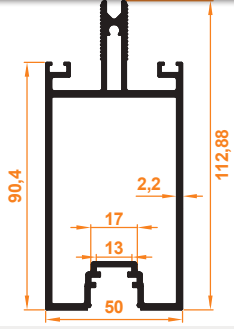
Led Kanallı Orta Kayıt Profili Center Mullion Profile with Led
