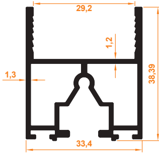
Fitilli Baza Profili Wicked Base Profile
