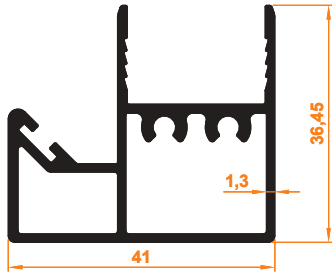
Kenet Baza Profil Interlocking Base Profile
