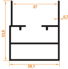
Star Kasa Profili Star Case Profile
