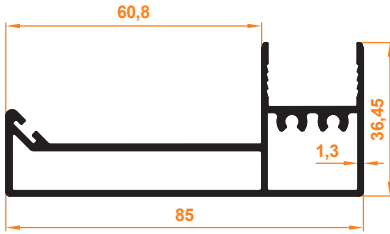
Geniş Kenet Baza Profil Wide Interlocking Base Profile
