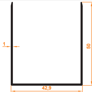
U Kapatma Profil U Closing Profile
