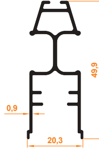
Nova Seri Kanat Profili Nova Wing Profile
