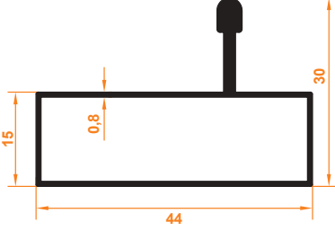
Platin Tekli Kasa Profil Platin Single Case Profile
