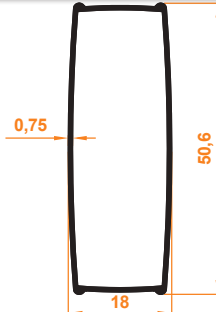
Ahşap Jaluzi Perde Etek Profili Venetian Blind Bottomrail Profile
