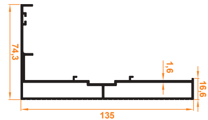
Yan Kasa Profil Side Frame Profile
