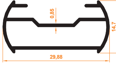
Aura Alt Kasa Profili Aura Bottom Case Profile
