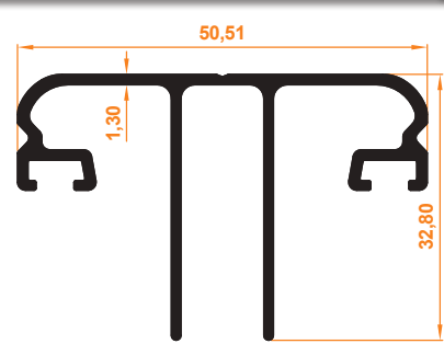
Cam Çita Profili Glass Strip Profile
