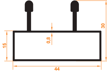
Platin Çiftli Kasa Profil Platin Double Case Profile
