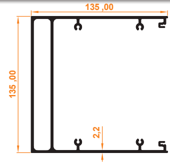
Gizli Ayak Profili Hidden Leg Profile
