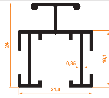
Çiftli Orta Profil Double Middle Profile
