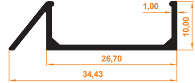
Junior Eşiksiz Kasa Profil Junior Case Profile without Threshold
