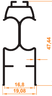
Dark Perde Kanat Profili Dark Blind Wing Profile
