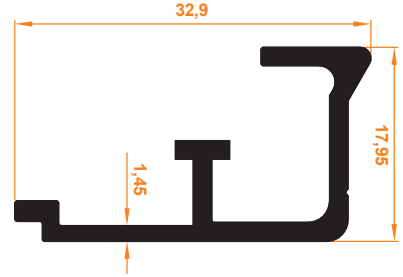
Yan Kasa Kapak Profili Side Case Cover Profile
