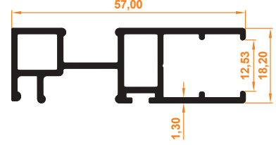
Platin Kanat Profil Platin Series Sash Profile
