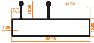
Platin Geniş Çiftli Kasa Profil Platin Wide Double Frame Profile
