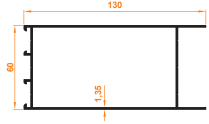
C60 Etek Profili C60 Skirt Profile
