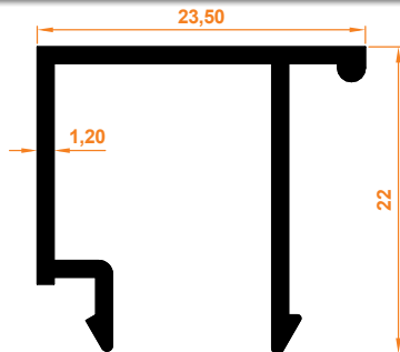
C60 Tek Cam Çıta Profili C60 Single Glass Stave Profile
