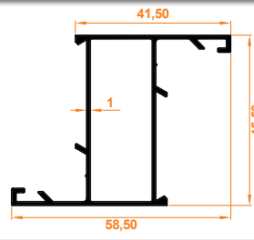
Aldoks (Dar) Kanat Profili Aldoks (Narrow) Airfoil
