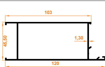
Aldoks Etek Profili Aldoks Skirt Profile
