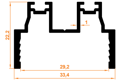
Düz Kapak Menteşe Profil Flat Cover with Hinge Profile
