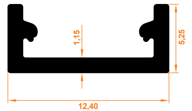
Kapatma Profil Closing Profile
