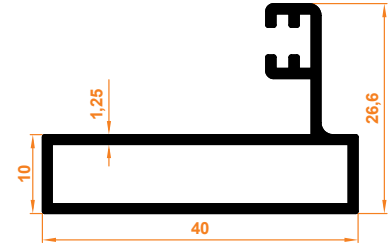
Dar Yan Dikme Thin Side Column
