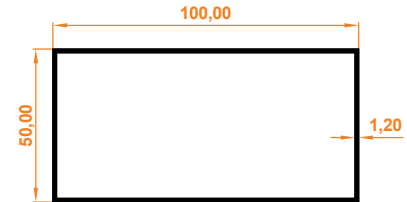
50x100x1,2 mm Kutu Profil 50x100x1,2 mm Box Profile
