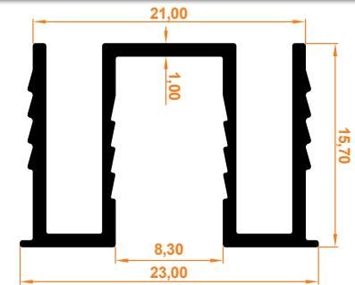
8 mm Cam Adaptörü 8mm Glass Adapter
