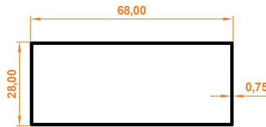
28x68 Kutu Profil 28x68 Box Profile
